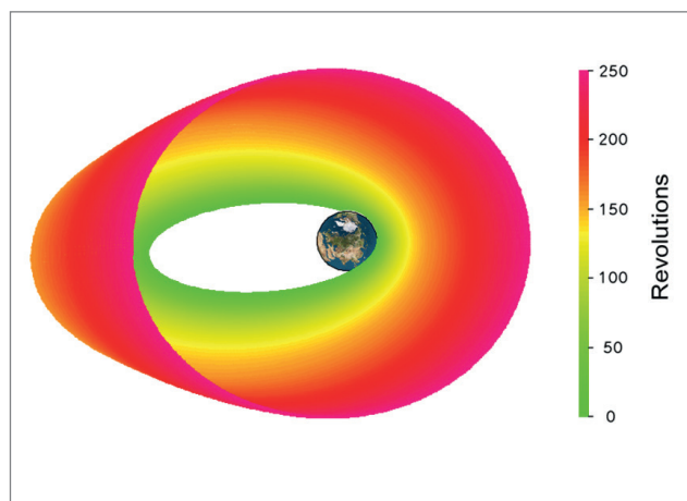
Optimal low thrust transfer from GTO to GEO
