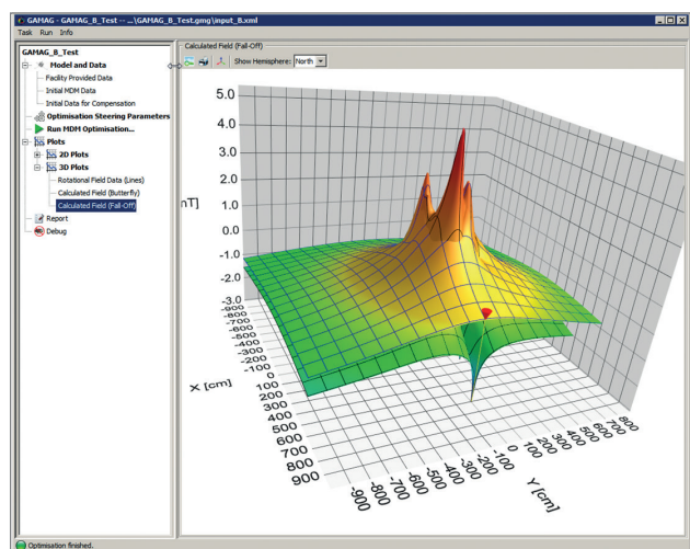
Magnetic field identification with GAMAG
