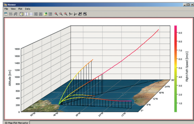
Ascent trajectories of launcher family
